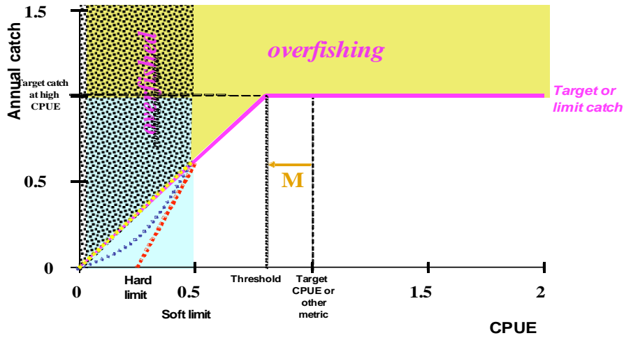
Figure 2: Information-limited default harvest strategy. The solid line is the harvest strategy decision rule. For a given recent CPUE, it specifies the annual catch that should be used as a basis for setting the TAC. The dotted lines represent different possible management responses when adopting a soft limit or a hard limit.
