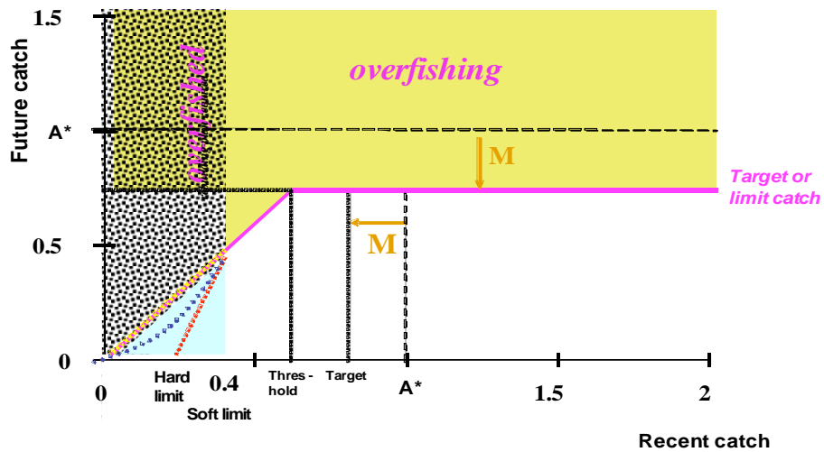
Figure 3: Information-deficient default harvest strategy. The solid line is the harvest strategy decision rule. For a given recent catch, it specifies the annual catch that should be used as a basis for setting the TAC. The dotted lines represent different possible management responses when adopting a soft limit or a hard limit.
