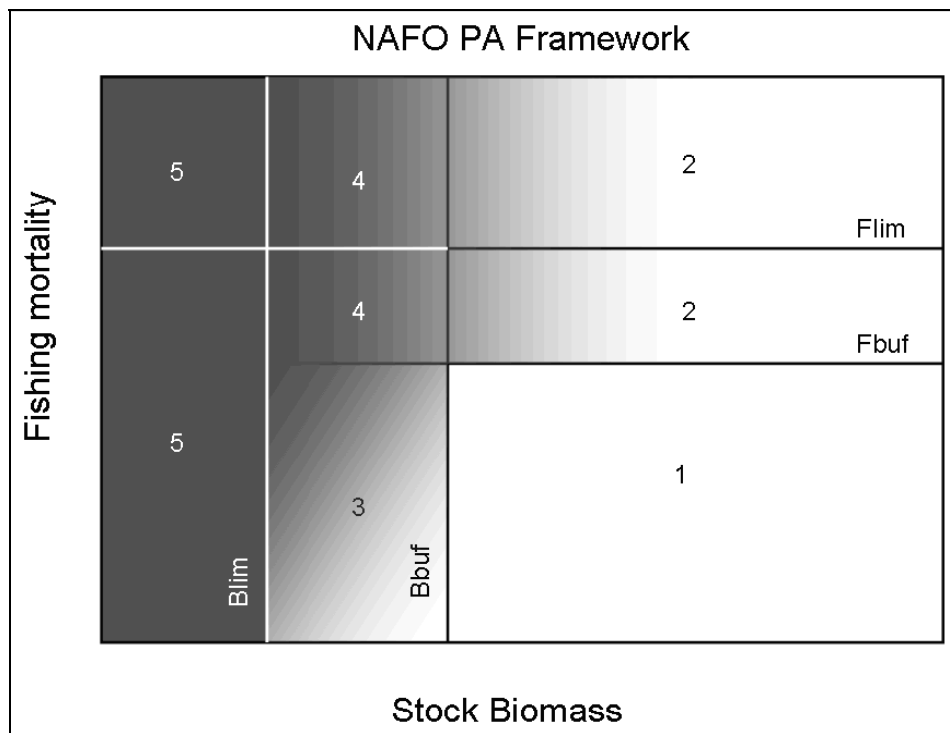
Figure 7: NAFO precautionary approach framework
